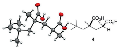
Figure 1. X-ray structure of 4.
